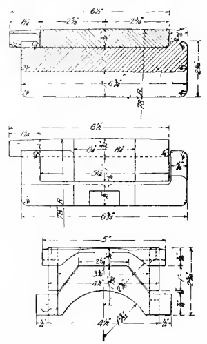
Figs. 5399-5401. WEDGE AND BEARING.
